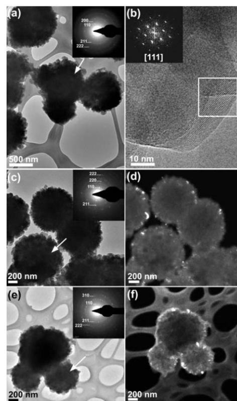
Fig. 7 TEM images of (a–b) SOD-16Et(2), (c–d) SOD-16Et(3), and (e–f) SOD-16Et(16). (b) is the HRTEM image captured on a shell sodalite nanocrystal. (d) and (f) are dark-field (DF) TEM images. The insets in panels (a), (c), and (e) are selected area electron diffraction (SAED) patterns collected from the entire particles as pointed by the arrows in each panel. The inset in panel (b) is the fast Fourier transform (FFT) pattern derived from the highlighted region in HRTEM image (b).
