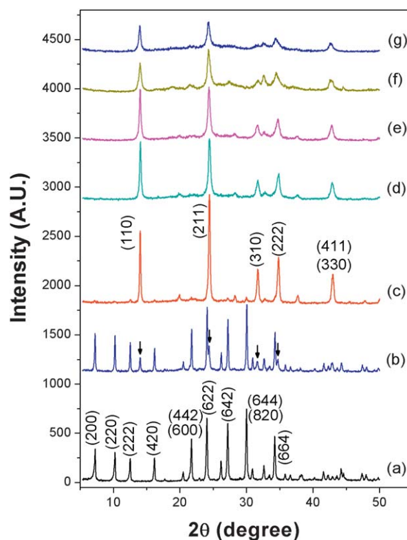
Fig. 1 XRD patterns of zeolite A (LTA) and sodalite (SOD) prepared with different amounts of water (Wt) and ethanol (Et) at 90^\circ\text{C} for t = 3-5 h. Spectra: (a) LTA-94Wt(3), (b) SOD-0Et(3), (c) SOD-0Et(5), (d) SOD-4Et(3), (e) SOD-8Et(3), (f) SOD-16Et(3), and (g) SOD-32Et(3). Spectra (a) and (c) are indexed to zeolite A and sodalite structures, respectively. The arrows in spectrum (b) indicate the emerging peaks of sodalite phase.
